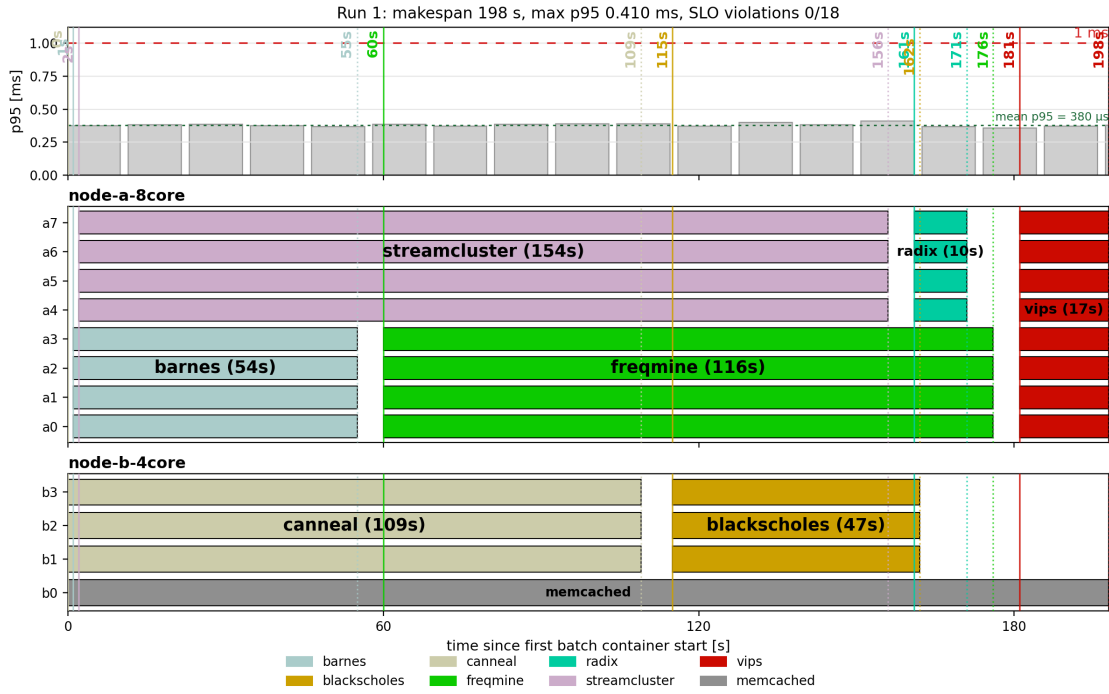
Run 1. AI-generated policy: memcached p95 latency and per-core placement; the red dashed line marks the 1 ms SLO.
