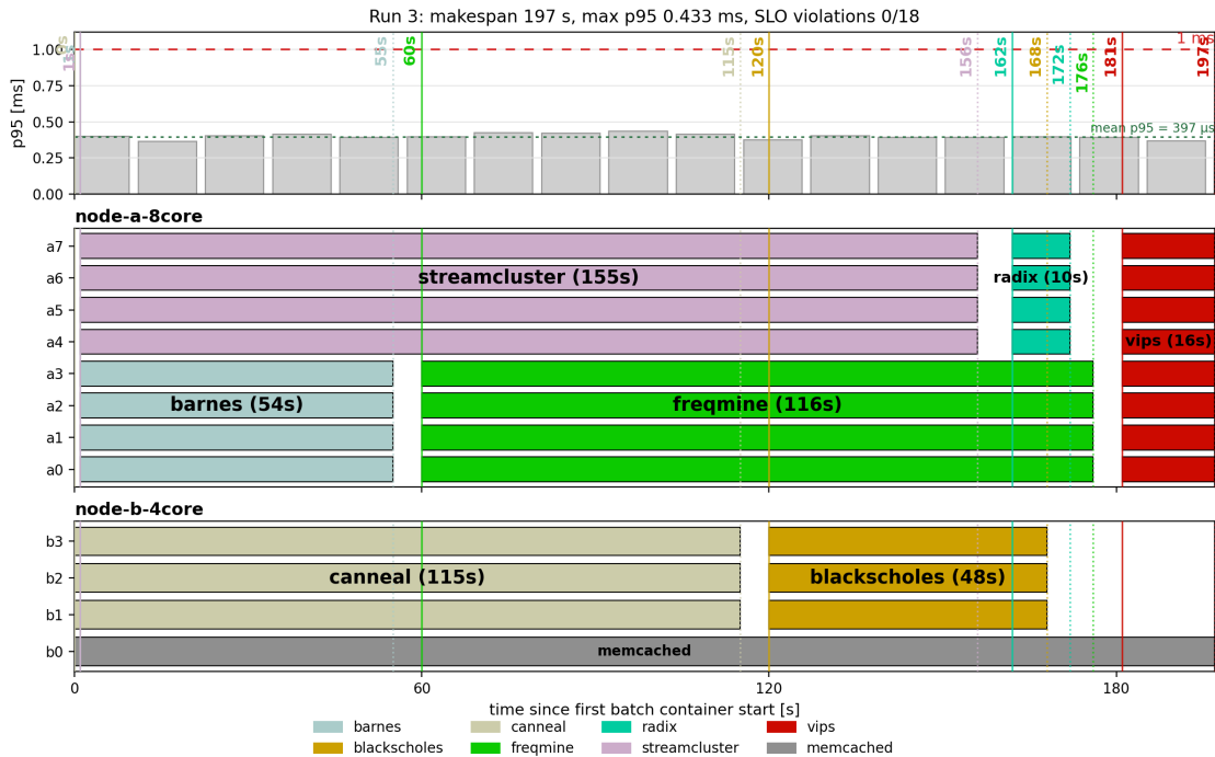
Run 3. AI-generated policy: memcached p95 latency and per-core placement; the red dashed line marks the 1 ms SLO.
